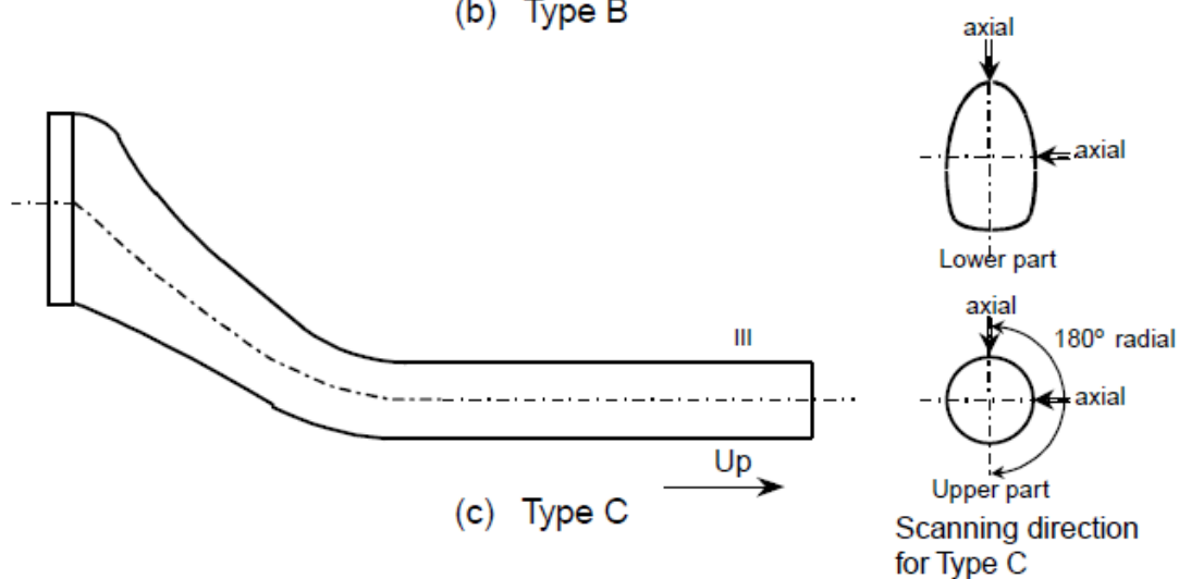
Fig. 2.5.2.3.3-4 Zones for ultrasonic testing on rudder stock
