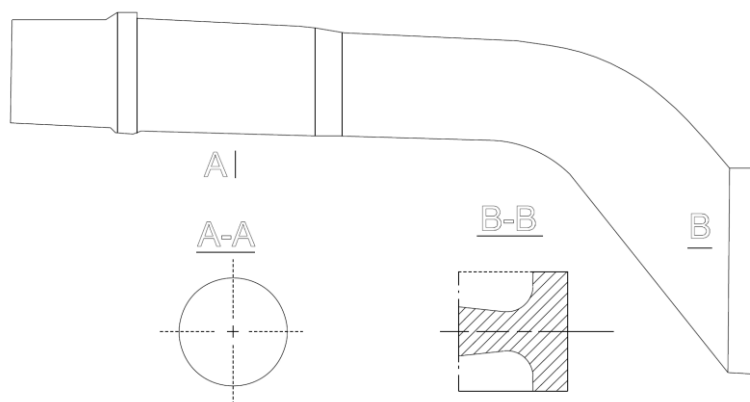
Fig. 2.5.2.4.1-2 Rudder stock.
