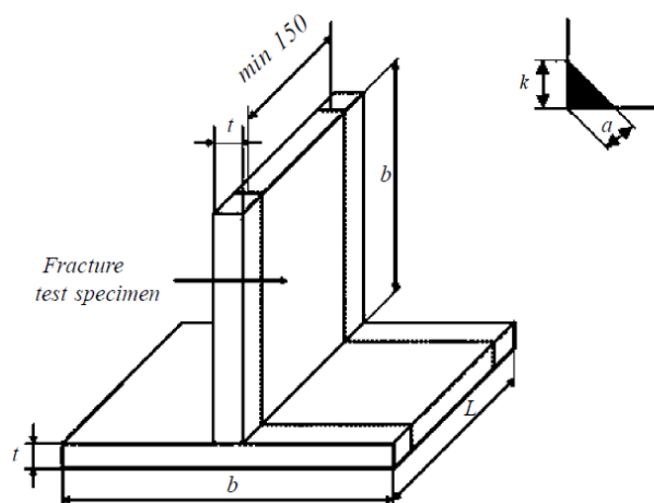
Fig. 2 Test piece of P 2 plate T-joint
