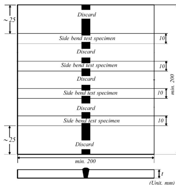
Fig. 1.2 Dimensions and types of test assembly for butt welds ( T ≥ 12 mm)
